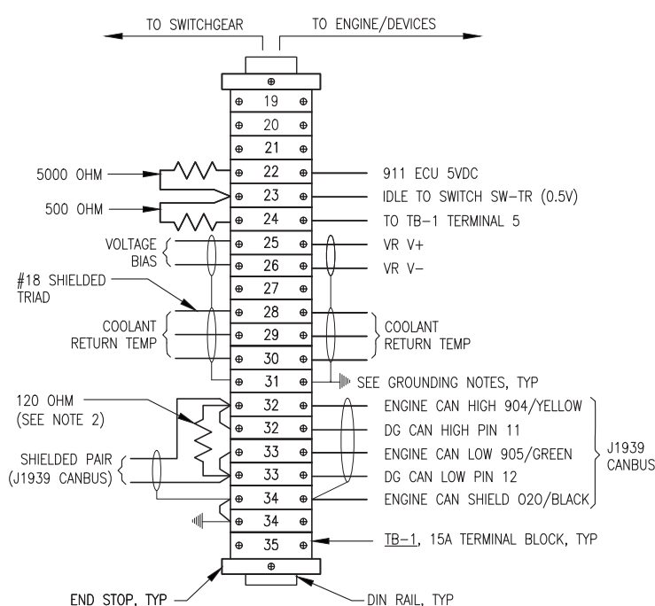
5 TERMINAL STRIP CONNECTIONS E3 NO SCALE
