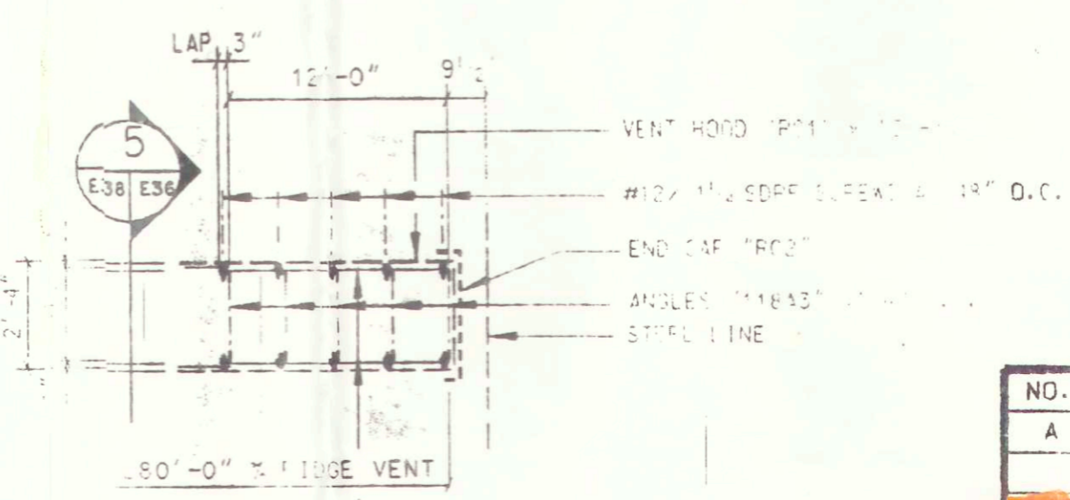
PARTIAL ERECTION PLAN OF RIDGE VENT
