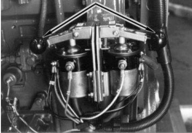
Fig. 12 - Manual Contactors
