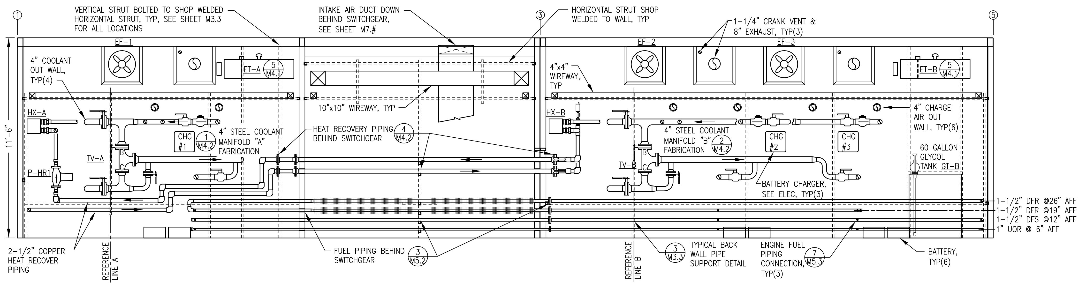
1 BACK WALL ELEVATION M3.1 3/8"=1'-0"
