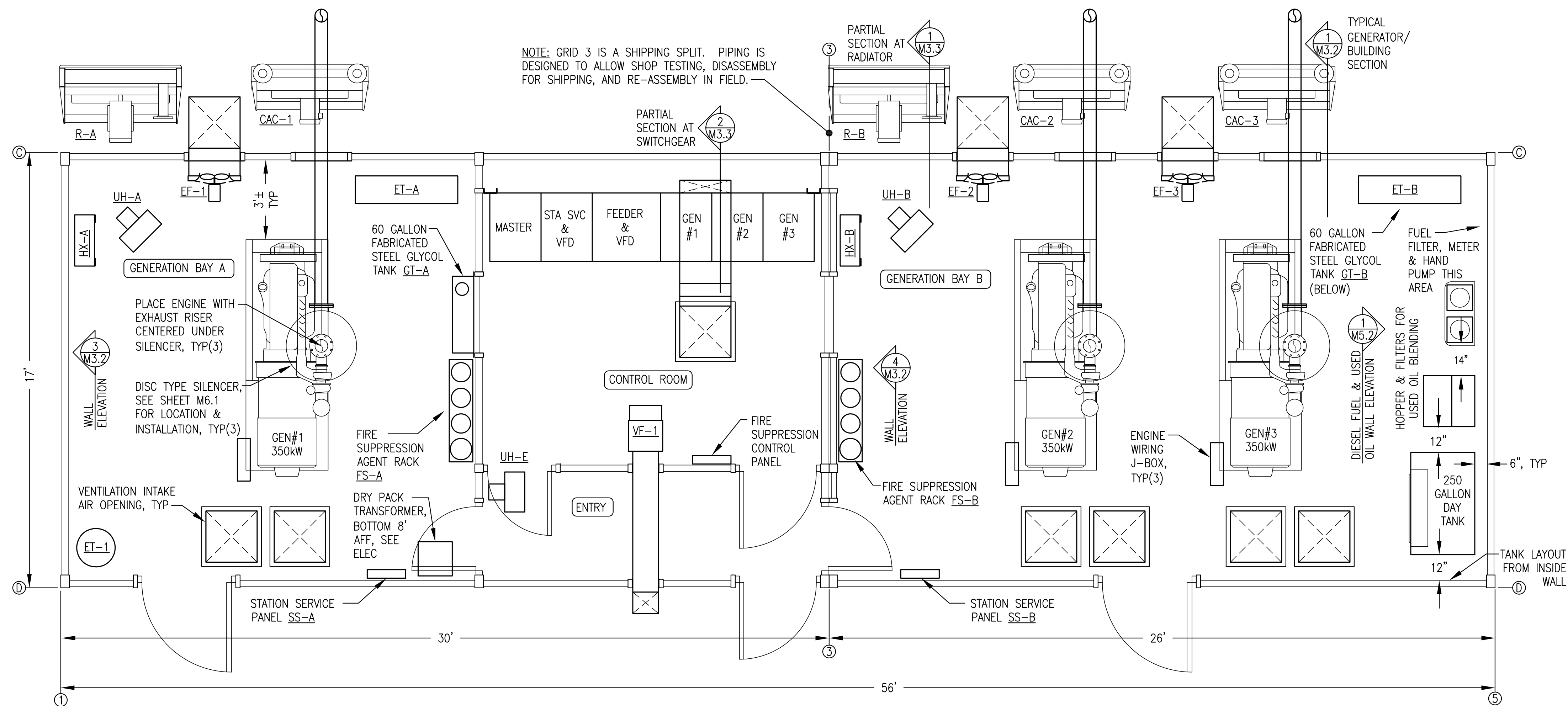
2 EQUIPMENT LAYOUT PLAN M3.1 3/8"=1'-0"
