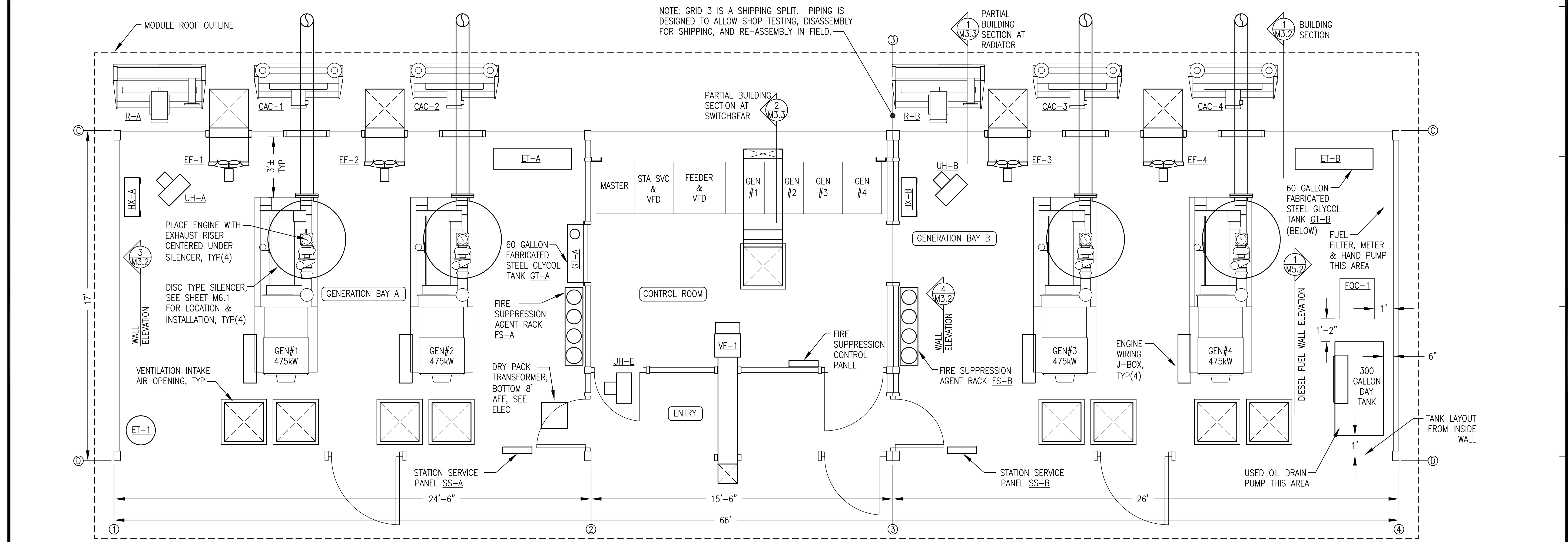
2 EQUIPMENT LAYOUT PLAN M3.1 3/8"=1'-0"
